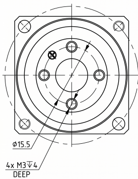
Mechanical View 3
