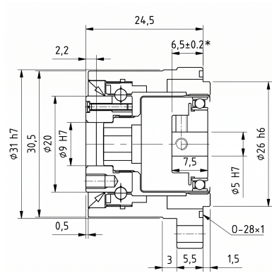
Mechanical View 1
