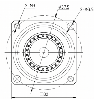
Mechanical View 2
