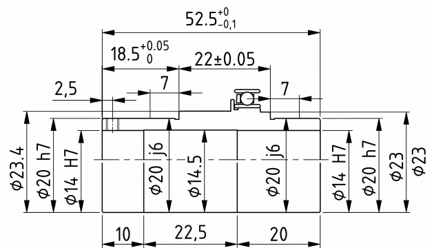
Mechanical View 4
