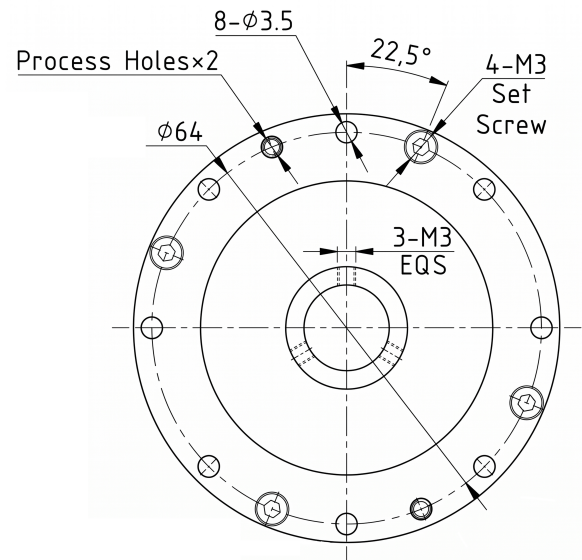
Mechanical View 2
