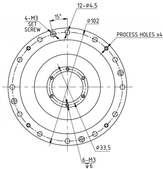
Mechanical View 3
