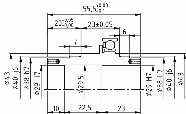
Mechanical View 4
