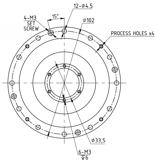
Mechanical View 3
