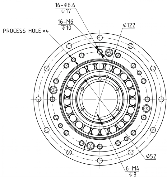
Mechanical View 1
