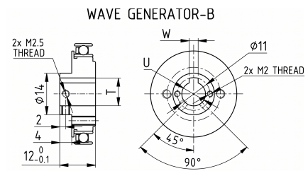
Mechanical View 4
