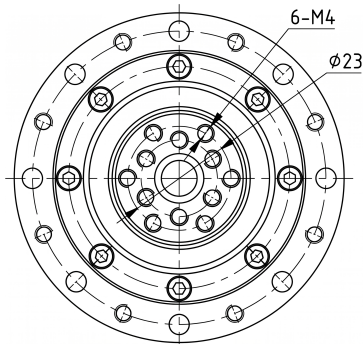
Mechanical View 3
