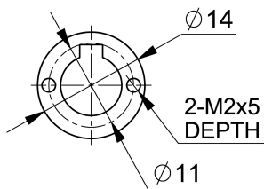
Mechanical View 5
