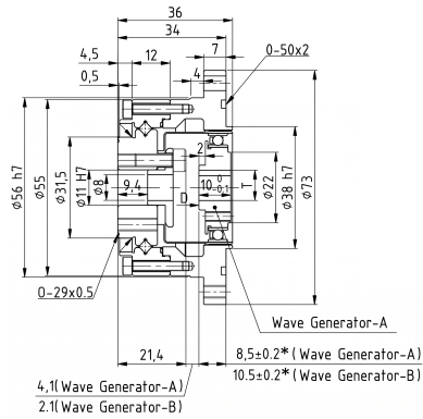
Mechanical View 1
