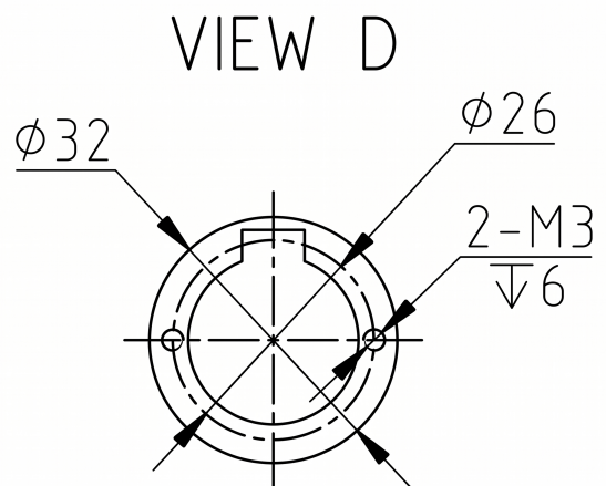
Mechanical View 4
