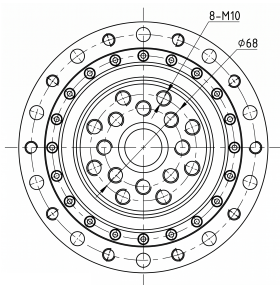
Mechanical View 3
