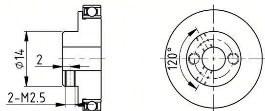
Mechanical View 4
