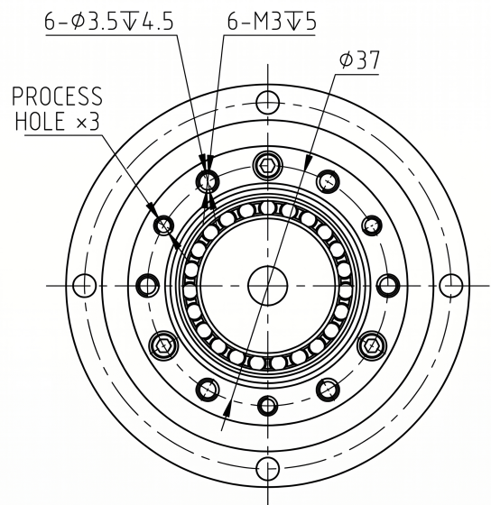
Mechanical View 3
