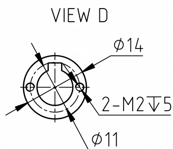
Mechanical View 5
