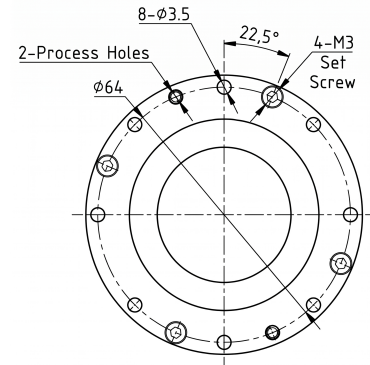
Mechanical View 2
