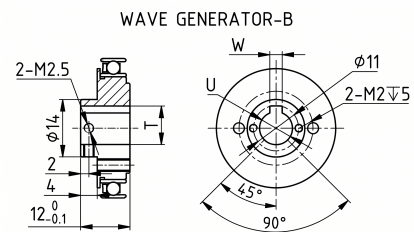
Mechanical View 4
