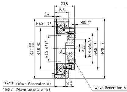
Mechanical View 1
