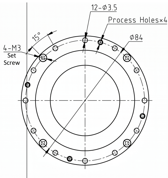
Mechanical View 3
