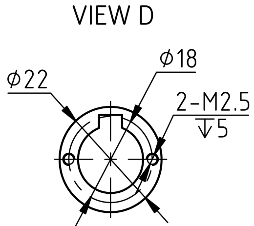
Mechanical View 4
