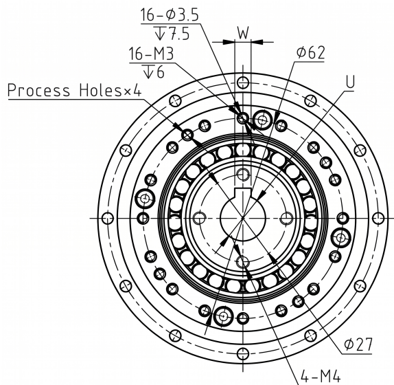
Mechanical View 1
