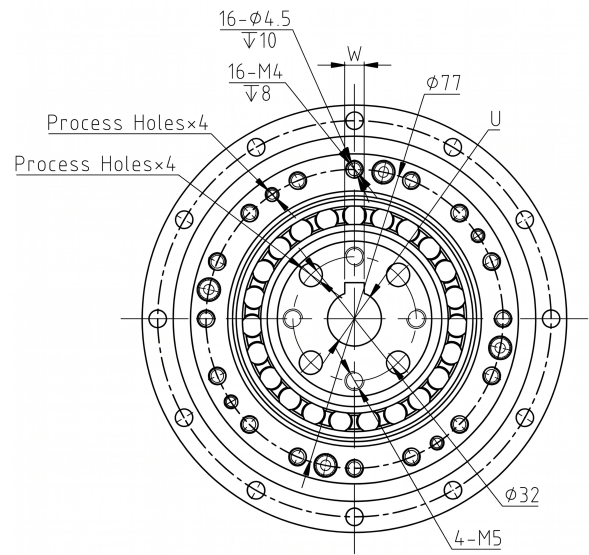
Mechanical View 2
