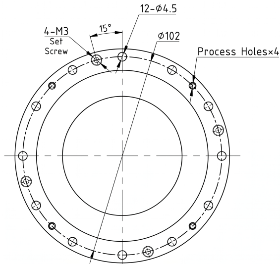
Mechanical View 1
