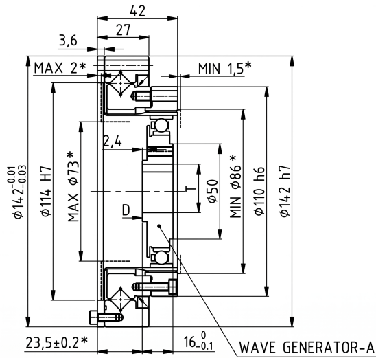
Mechanical View 1
