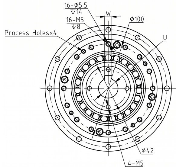
Mechanical View 2
