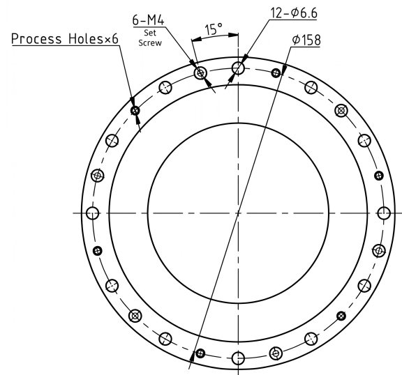
Mechanical View 2
