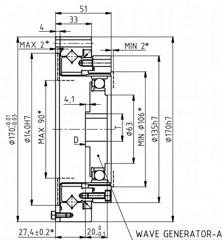
Mechanical View 3
