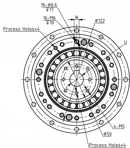
Mechanical View 1
