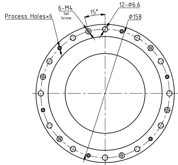
Mechanical View 2
