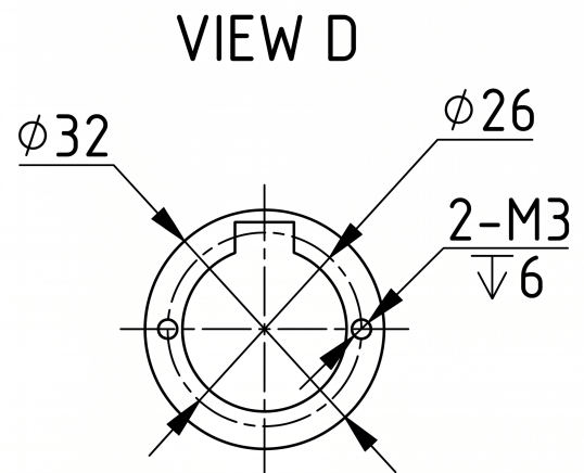
Mechanical View 4
