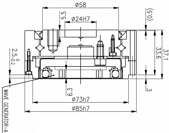
Mechanical View 1
