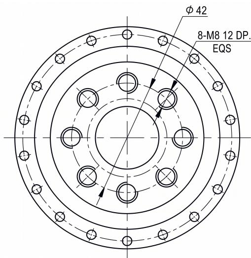
Mechanical View 3
