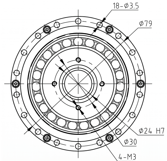
Mechanical View 2
