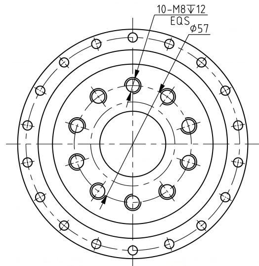
Mechanical View 2
