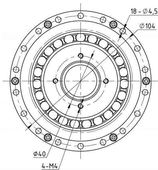
Mechanical View 3
