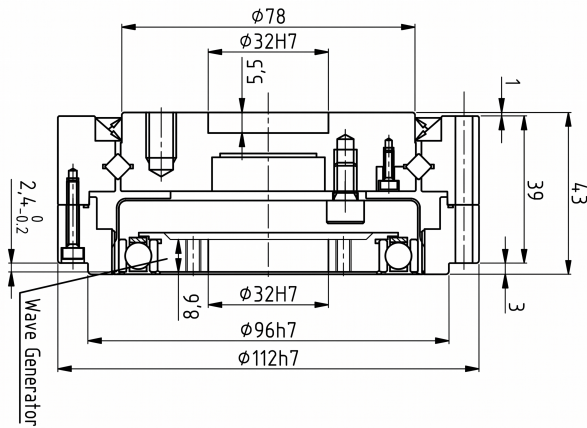
Mechanical View 1
