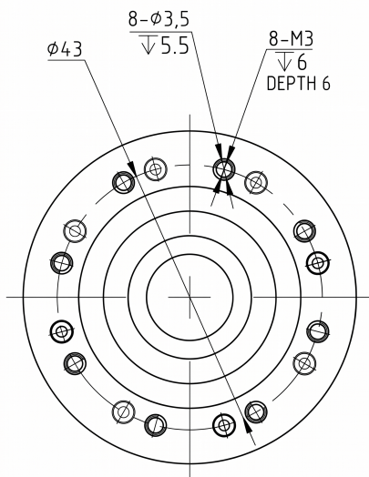
Mechanical View 3
