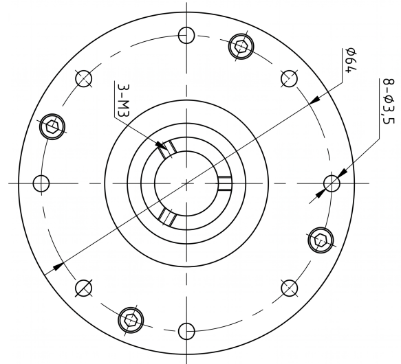
Mechanical View 2
