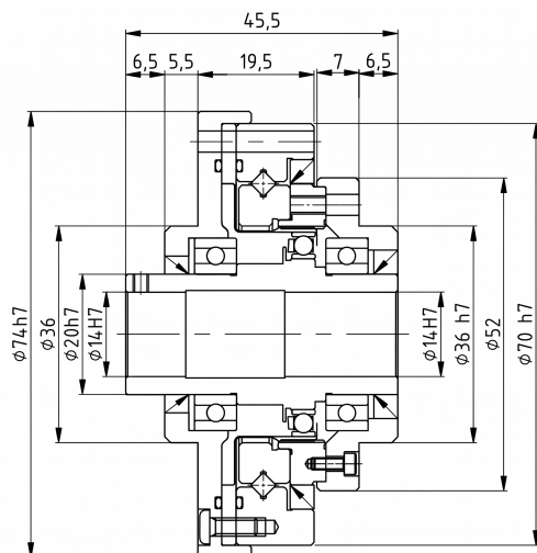
Mechanical View 1
