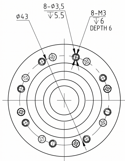
Mechanical View 3
