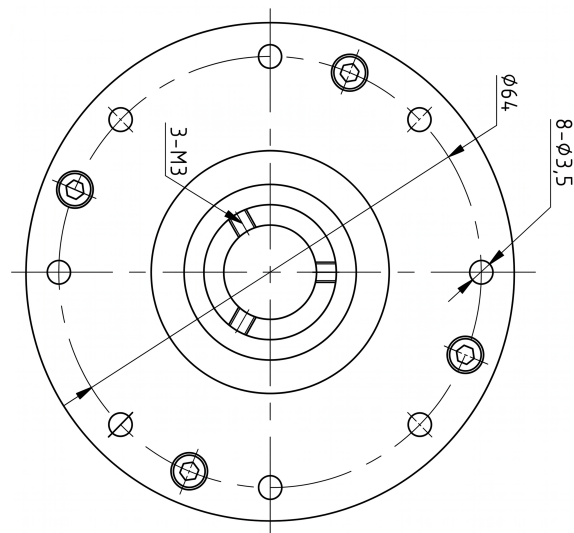
Mechanical View 2
