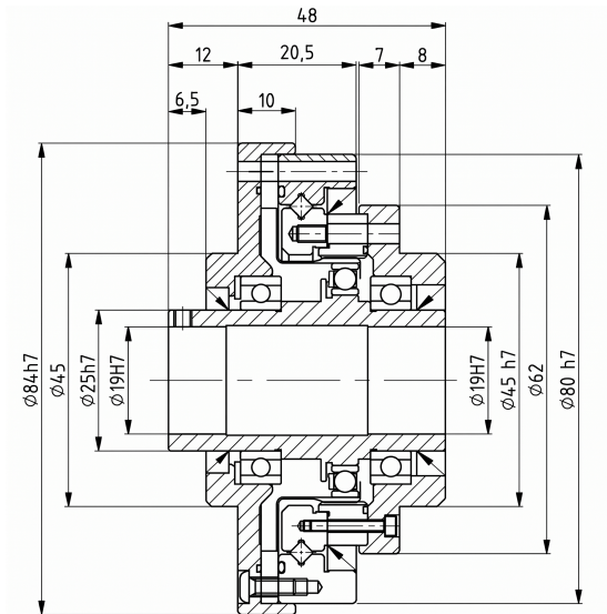
Mechanical View 1
