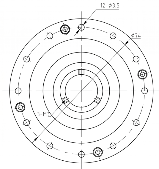
Mechanical View 3
