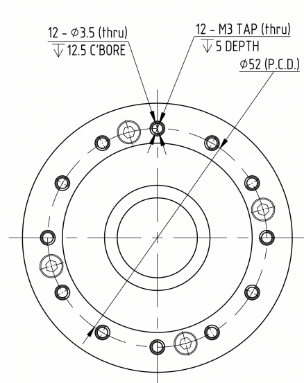
Mechanical View 2
