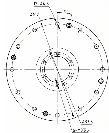
Mechanical View 2
