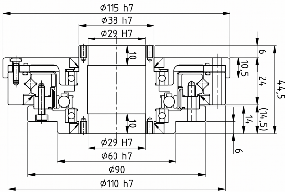
Mechanical View 1
