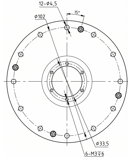
Mechanical View 2
