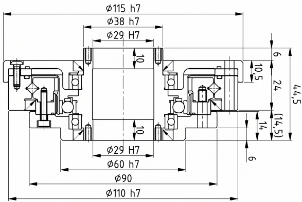
Mechanical View 1
