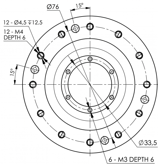
Mechanical View 3
