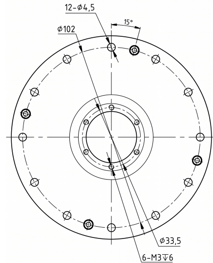
Mechanical View 2
