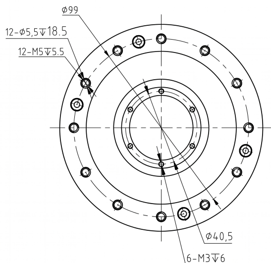
Mechanical View 3
