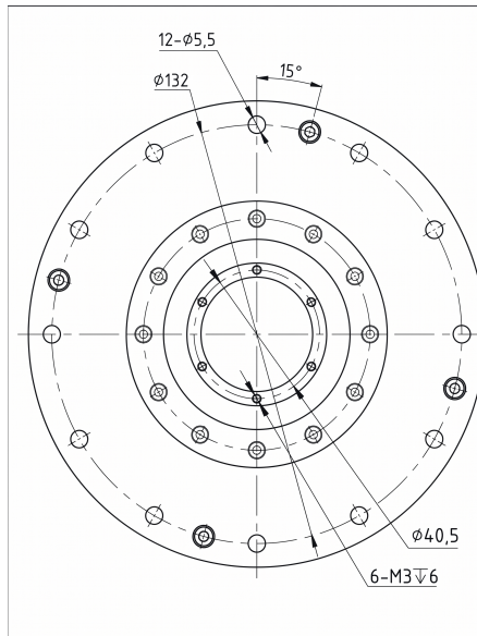
Mechanical View 1
