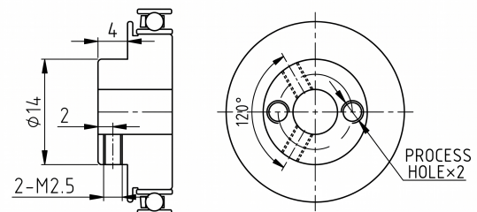
Mechanical View 4
