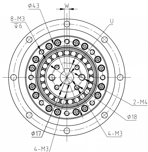
Mechanical View 3
