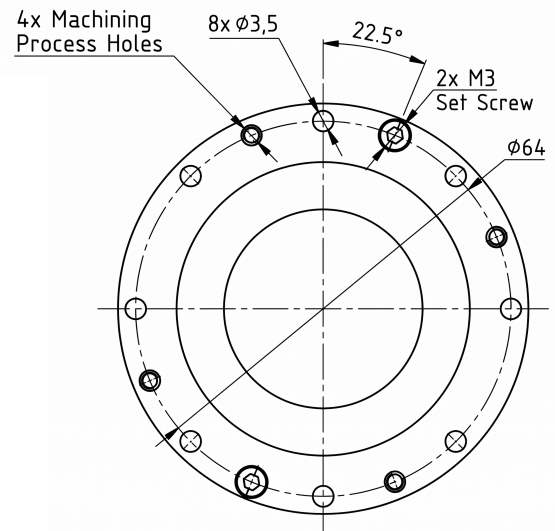
Mechanical View 2
