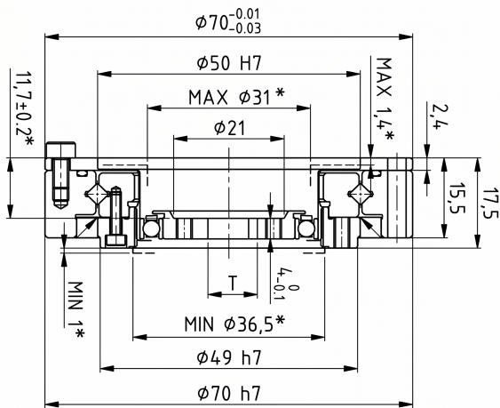
Mechanical View 1
