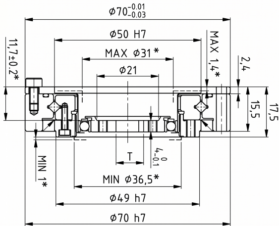
Mechanical View 1
