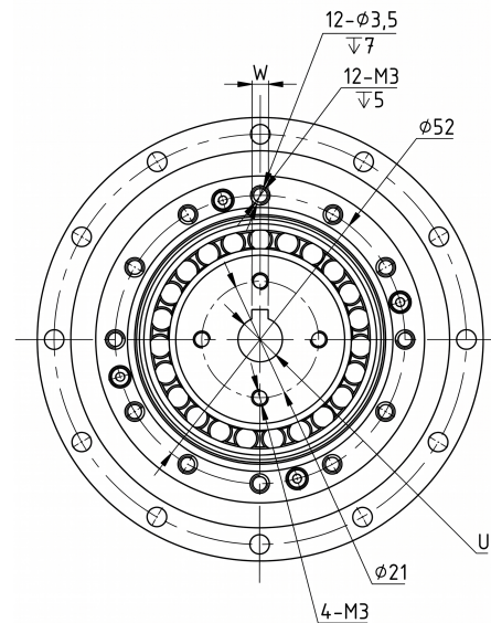
Mechanical View 2
