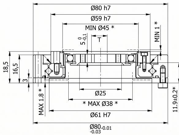
Mechanical View 1
