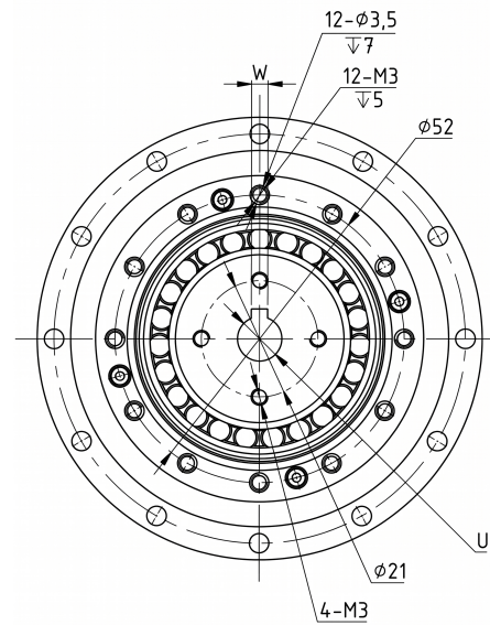
Mechanical View 2
