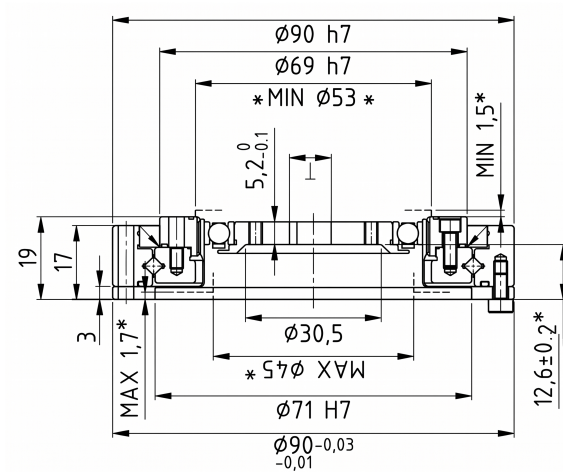
Mechanical View 3
