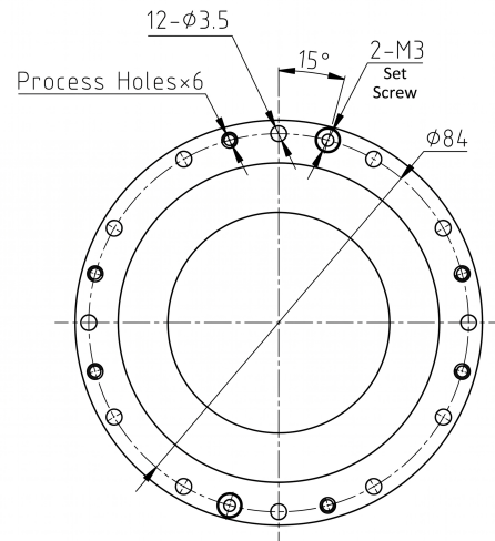
Mechanical View 2
