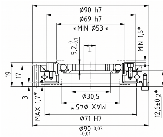
Mechanical View 3
