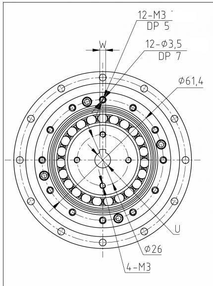
Mechanical View 1
