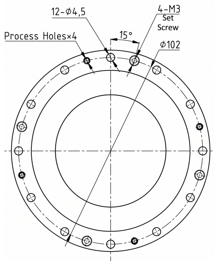
Mechanical View 3
