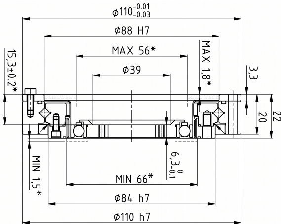
Mechanical View 1
