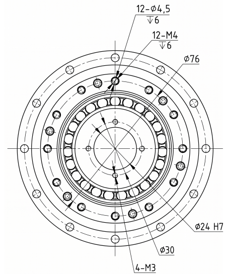
Mechanical View 2
