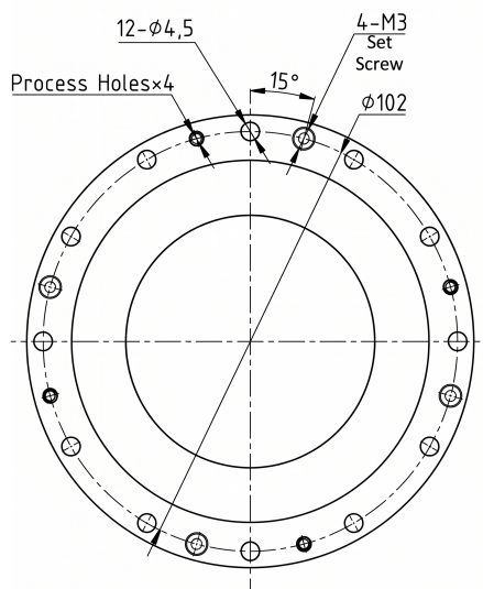
Mechanical View 3
