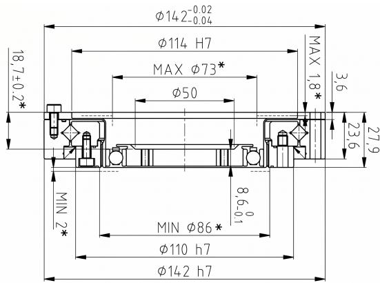
Mechanical View 1
