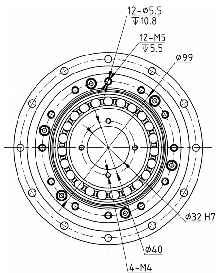
Mechanical View 3
