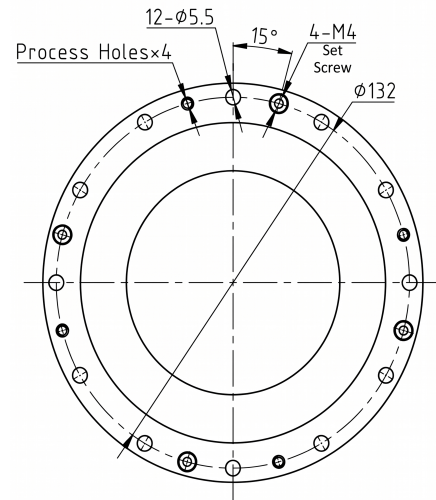
Mechanical View 2
