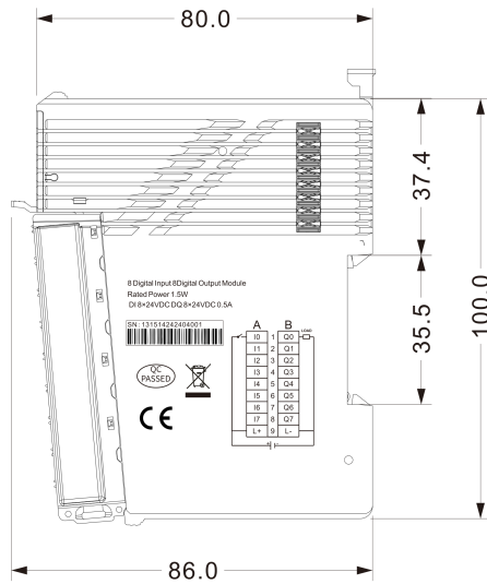
Mechanical View 1
