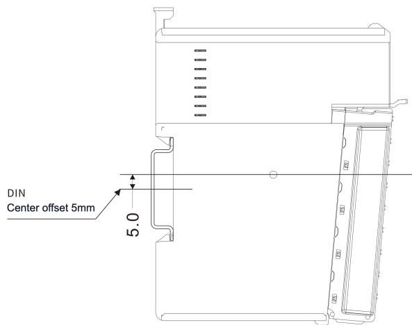
Mechanical View 3
