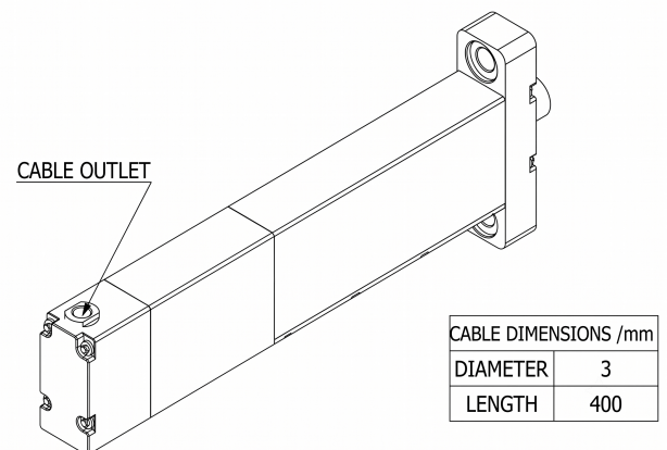
Mechanical View 4
