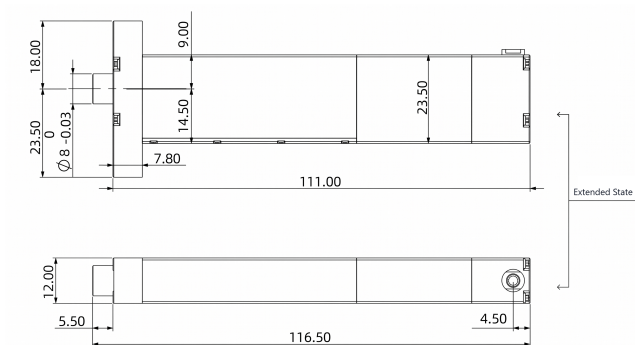
Mechanical View 3
