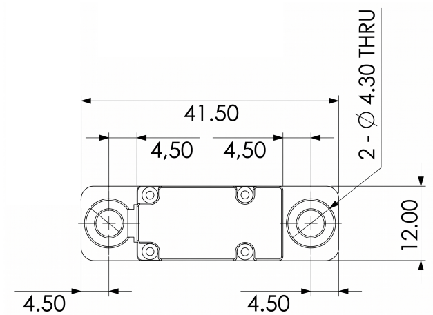
Mechanical View 1
