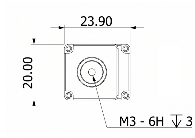
Mechanical View 3
