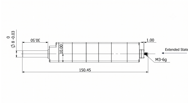
Mechanical View 1
