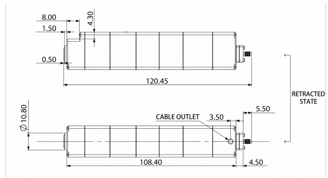
Mechanical View 4
