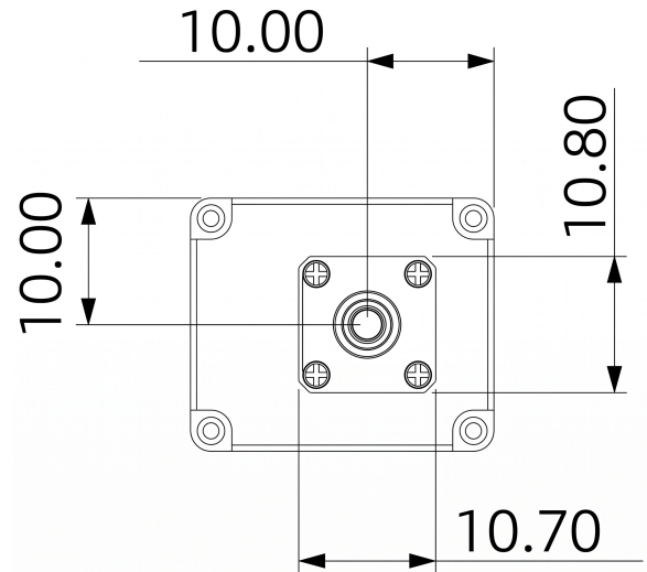
Mechanical View 2
