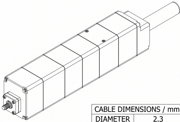
Mechanical View 5
