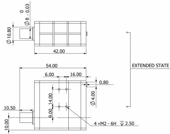
Mechanical View 1
