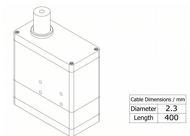
Mechanical View 4
