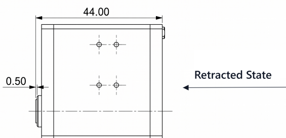
Mechanical View 5
