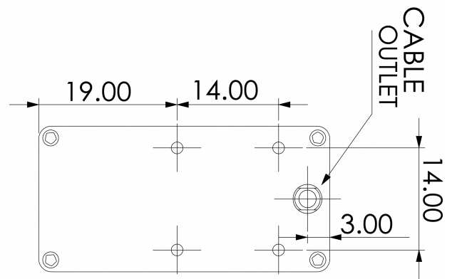
Mechanical View 2
