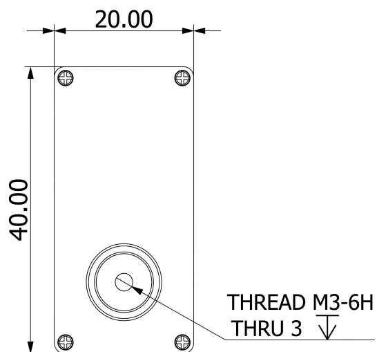
Mechanical View 3
