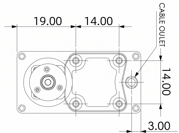
Mechanical View 2
