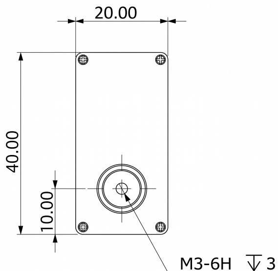
Mechanical View 3
