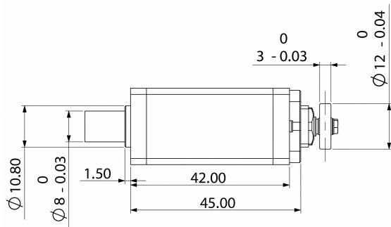
Mechanical View 1
