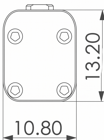
Mechanical View 3
