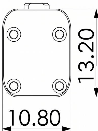
Mechanical View 3
