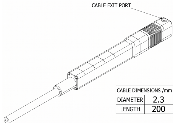
Mechanical View 4
