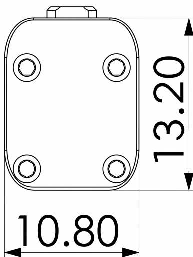
Mechanical View 3
