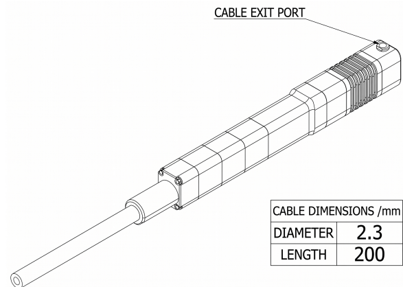
Mechanical View 4
