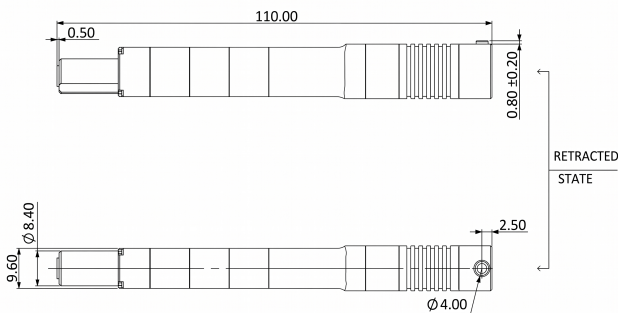
Mechanical View 5
