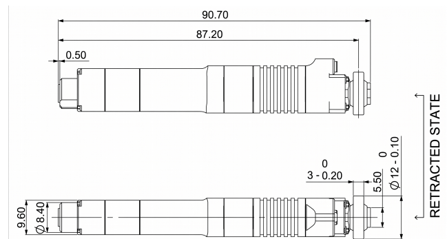
Mechanical View 4
