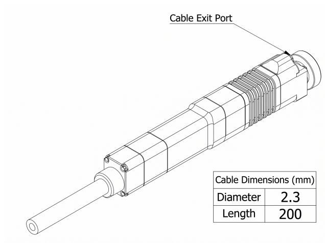
Mechanical View 5
