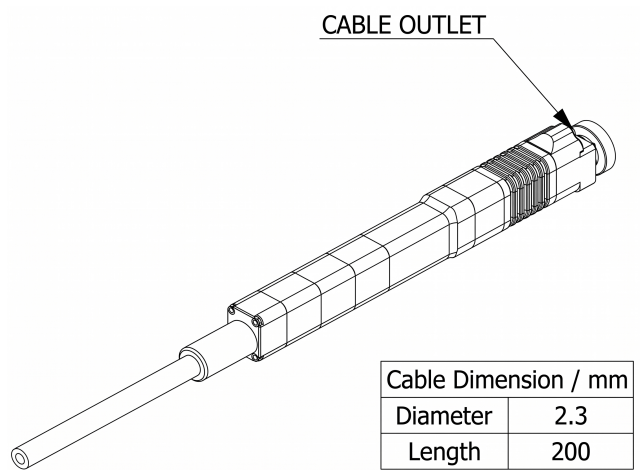
Mechanical View 5
