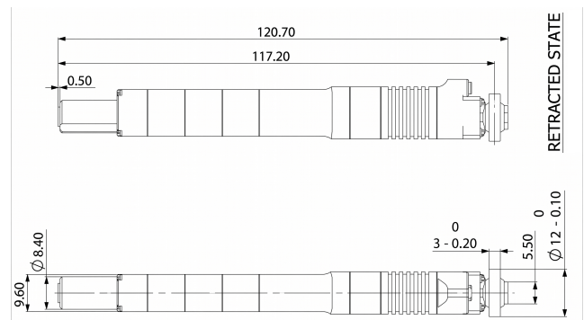
Mechanical View 4
