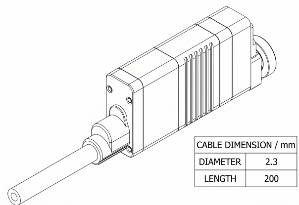
Mechanical View 4
