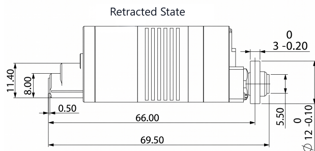
Mechanical View 5
