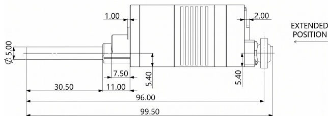
Mechanical View 3
